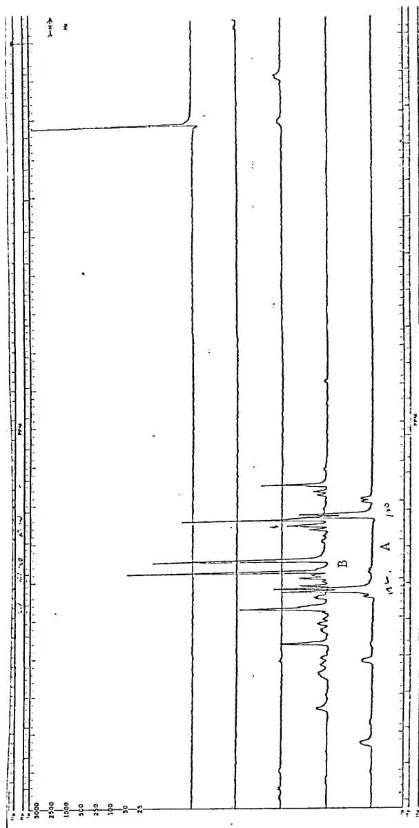
Figure 33 - F_{19} NMR of CF_2CFCl=CHCl_3 CF_2CFCl=CHCl_3
